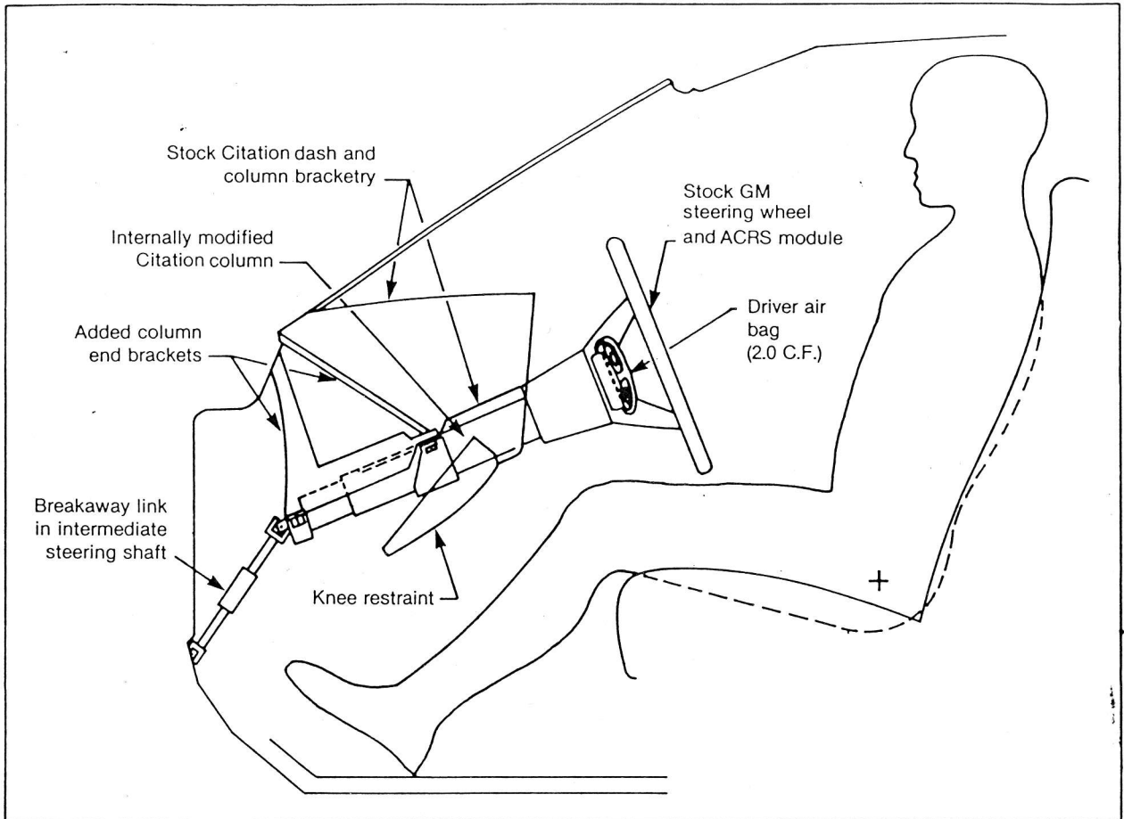
Figure 14. Citation driver system layout.
