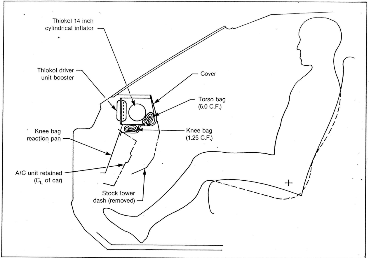
Figure 12. Citation passenger system layout.
